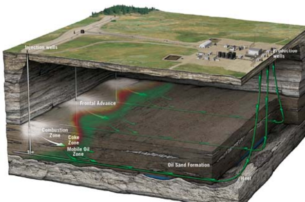
THAI Process: Photo Courtesy of Petrobank Energy and Resources Ltd.
