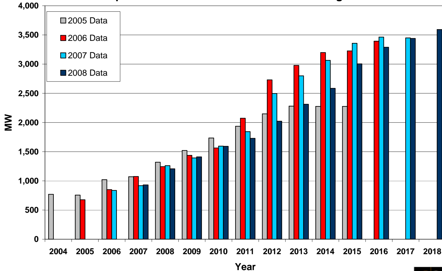
4-Year Forecast Comparison Oil Sands Co-generation Expected On-Site Power Demand - Mid Range
