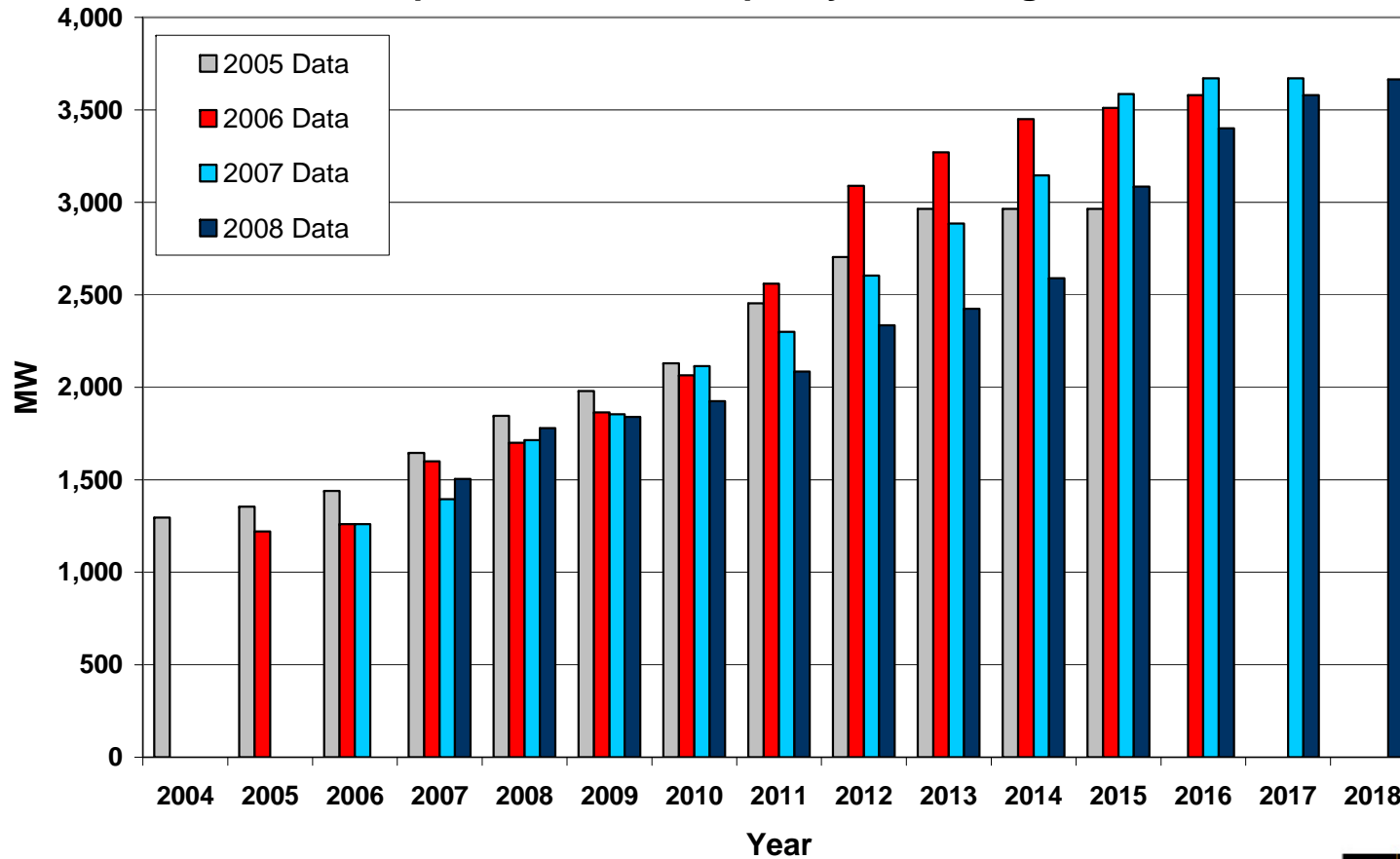
4-Year Forecast Comparison Oil Sands Co-generation Expected Installed Capacity - Mid Range
