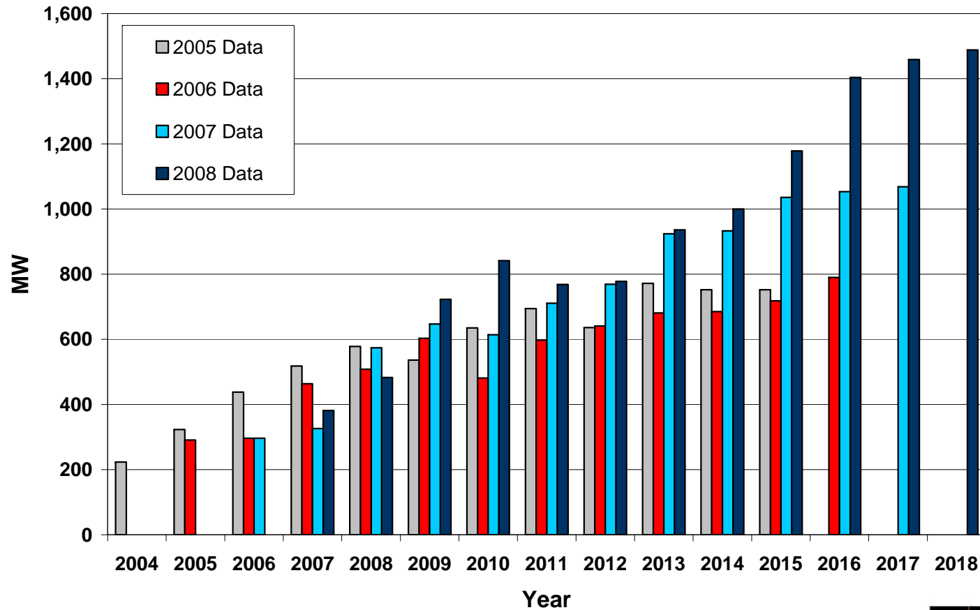
4-Year Forecast Comparison Oil Sands Co-generaton Stand-by Power Required from the Grid - Mid Range
